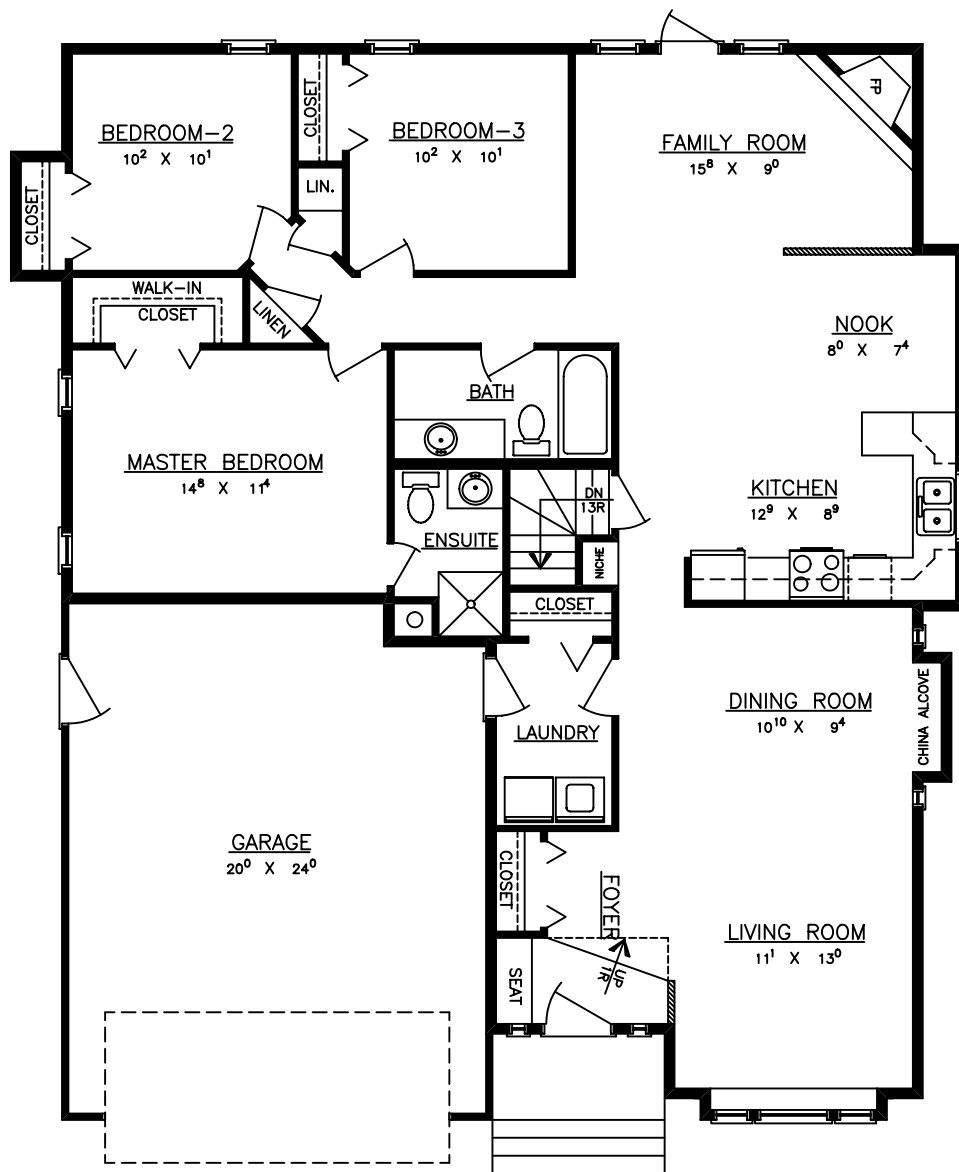
FLOOR PLAN
